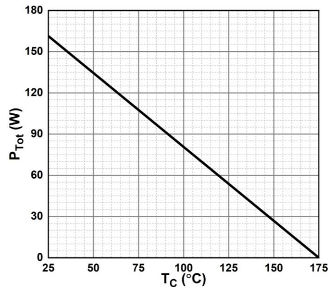
Figure 6. Power Derating
